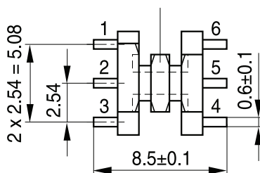
Terminals 2 and 5 are omitted in 4-terminal version
